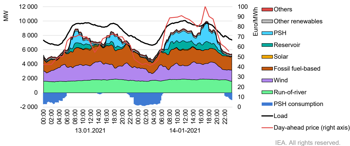
Figure 4.6 Austria hourly electricity dispatch, 13-14 January 2021
