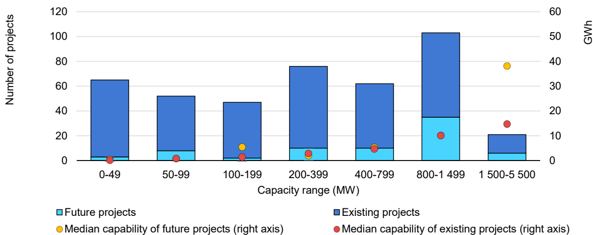
Figure 4.13 PSH storage capacity of existing and forecast plants, by generation capacity range
