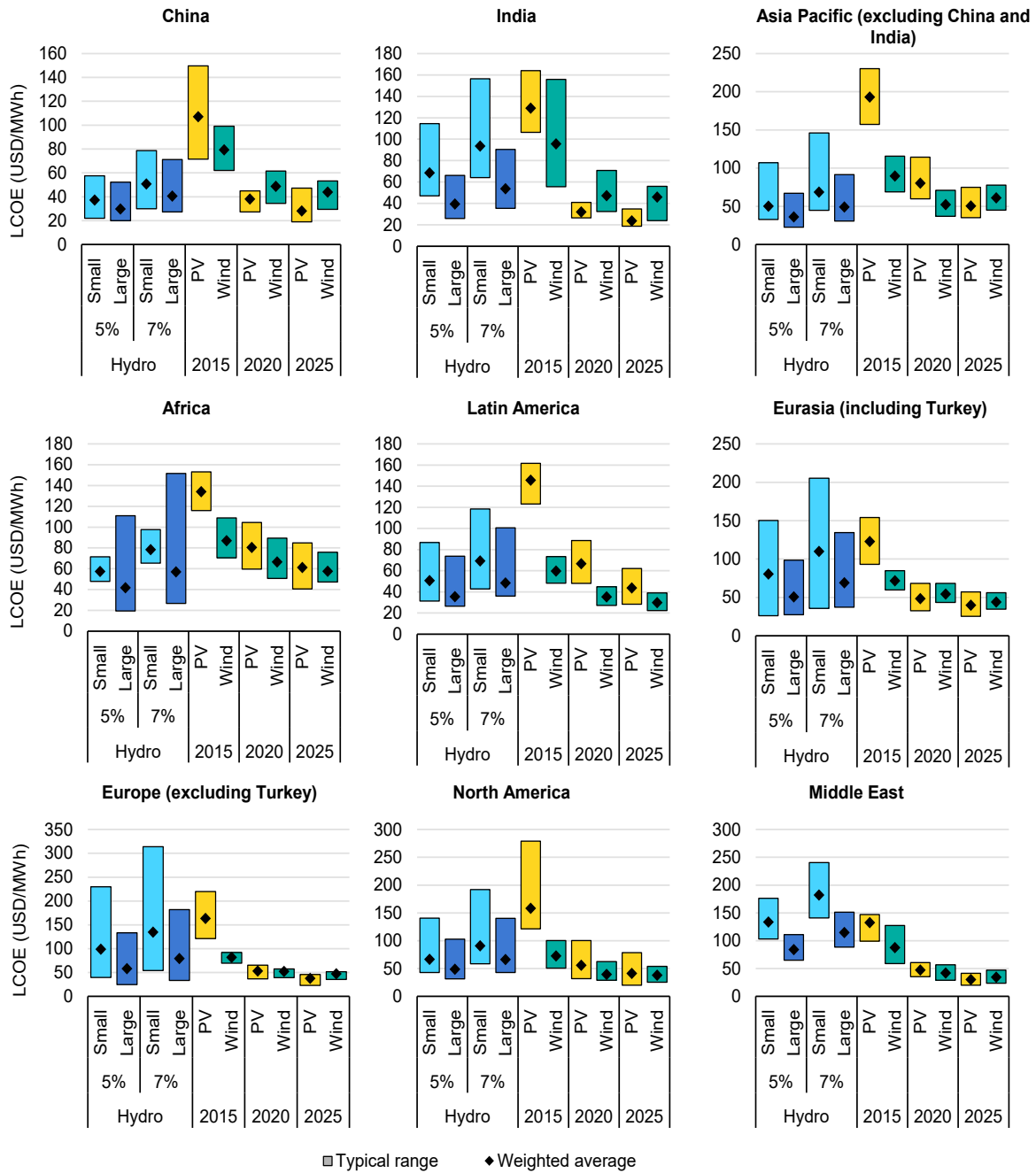
Figure 2.4 Average LCOE of new greenfield hydropower plants at 5% and 7% WACC (real), onshore wind and utility-scale PV, by region
