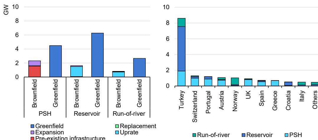
Figure 3.12 Europe net hydropower capacity additions, 2021-2030
