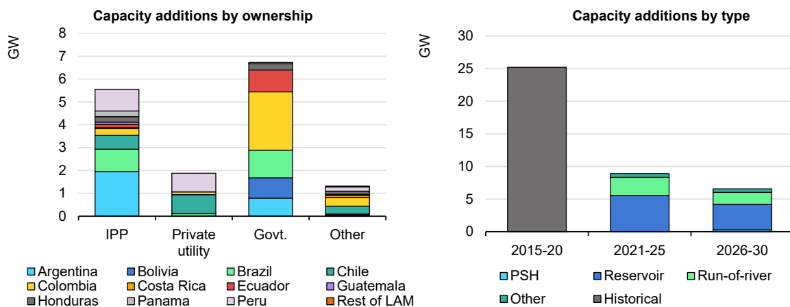
Figure 3.11 Latin America hydropower forecast summary
